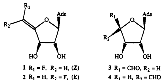
Figure 1. Structures of inhibitors of AdoHcy hydrolase.
